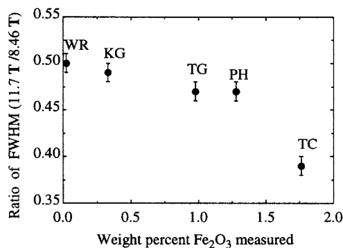
Figure 6. Ratio of FWHM measured in ppm at 11.7 T and 8.46 T plotted versus the weight percent Fe 2 O 3 . Vertical error bars denote the range of values observed after repeated measurements of the geode kaolinite (WR).
